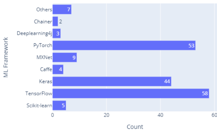
Fig. 12 Commonly Used ML Frameworks for Application development
