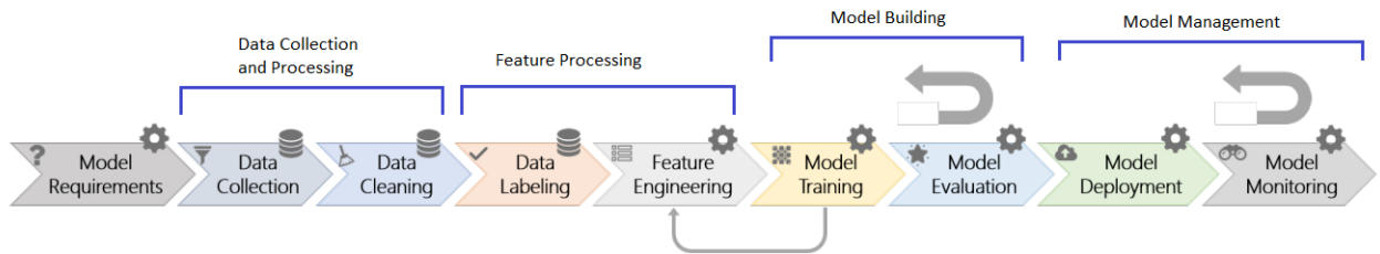
Fig. 1 Phases of ML workflow (adopted from Amershi et al. [1])
