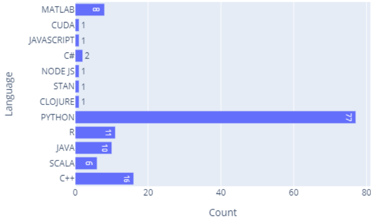
Fig. 9 Programming Languages for ML Development
